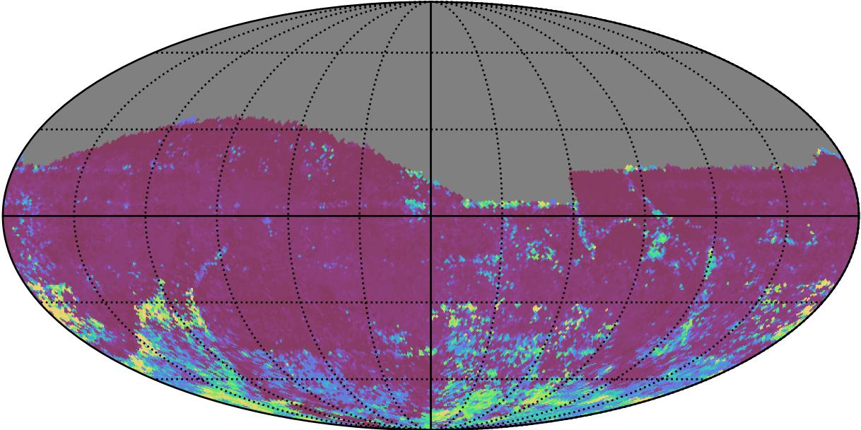
too_elab_heavy_r64_d3_griz_v3.4_10yrs All sky i band: 75th Percentile Intranight Timespan
