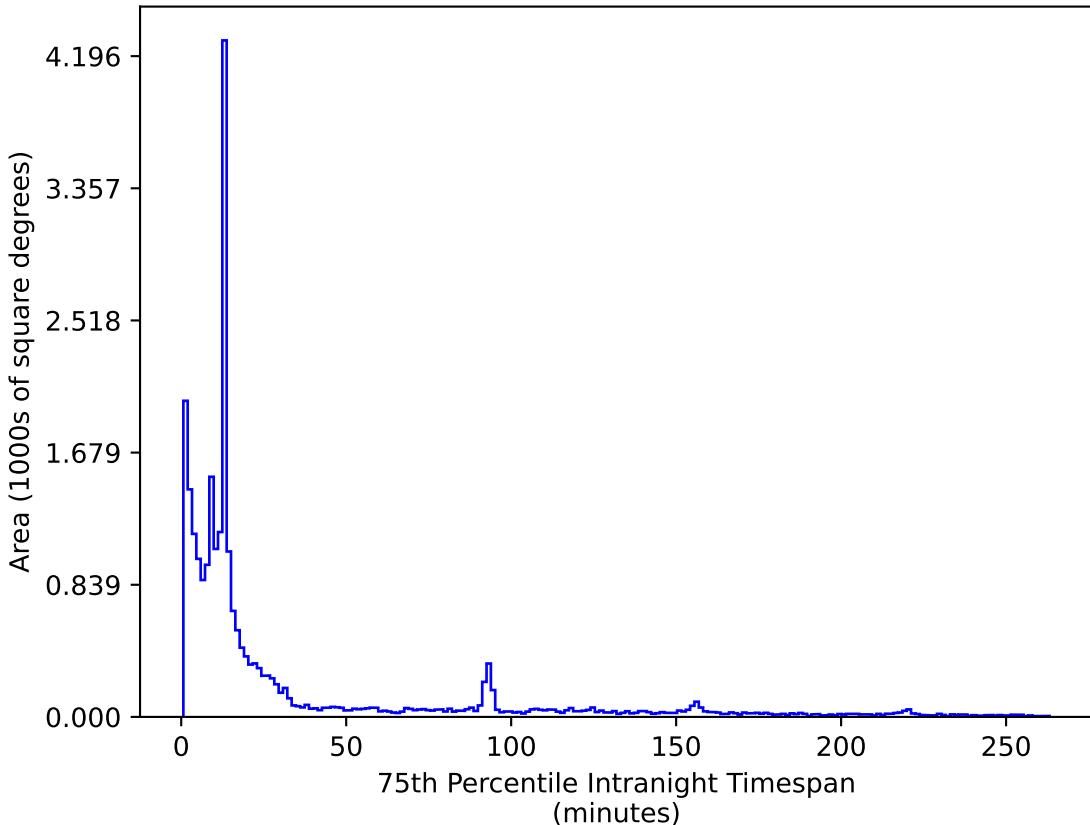
too_elab_heavy_r64_d3_griz_v3.4_10yrs All sky i band: 75th Percentile Intranight Timespan
