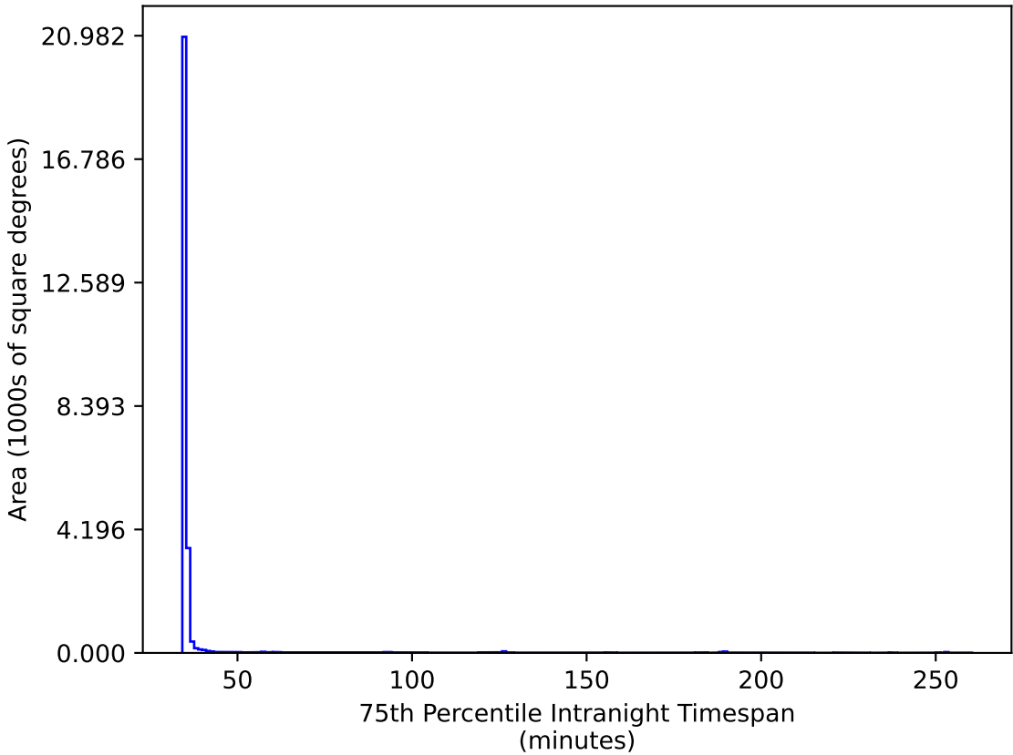
too_elab_heavy_r64_d3_griz_v3.4_10yrs All sky gr bands: 75th Percentile Intranight Timespan
