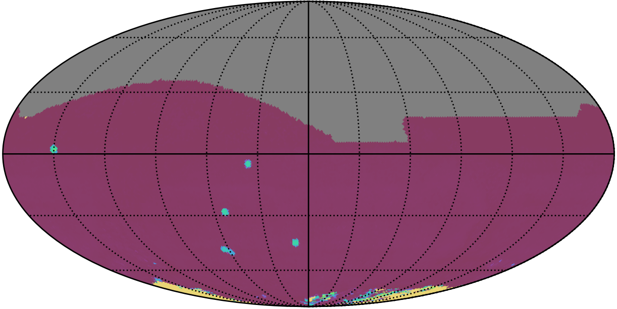
too_elab_heavy_r64_d3_griz_v3.4_10yrs All sky all bands: 75th Percentile Intranight Timespan
