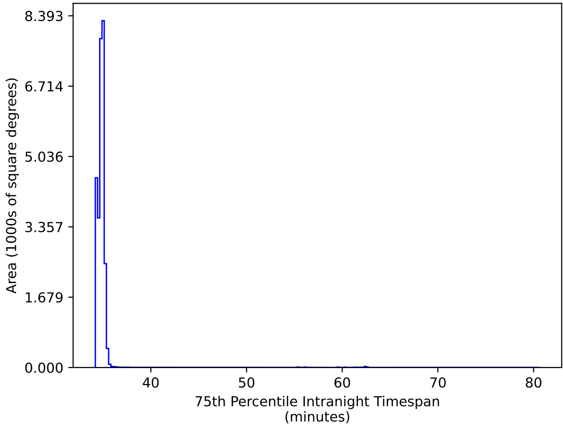
too_elab_heavy_r64_d3_griz_v3.4_10yrs All sky all bands: 75th Percentile Intranight Timespan
