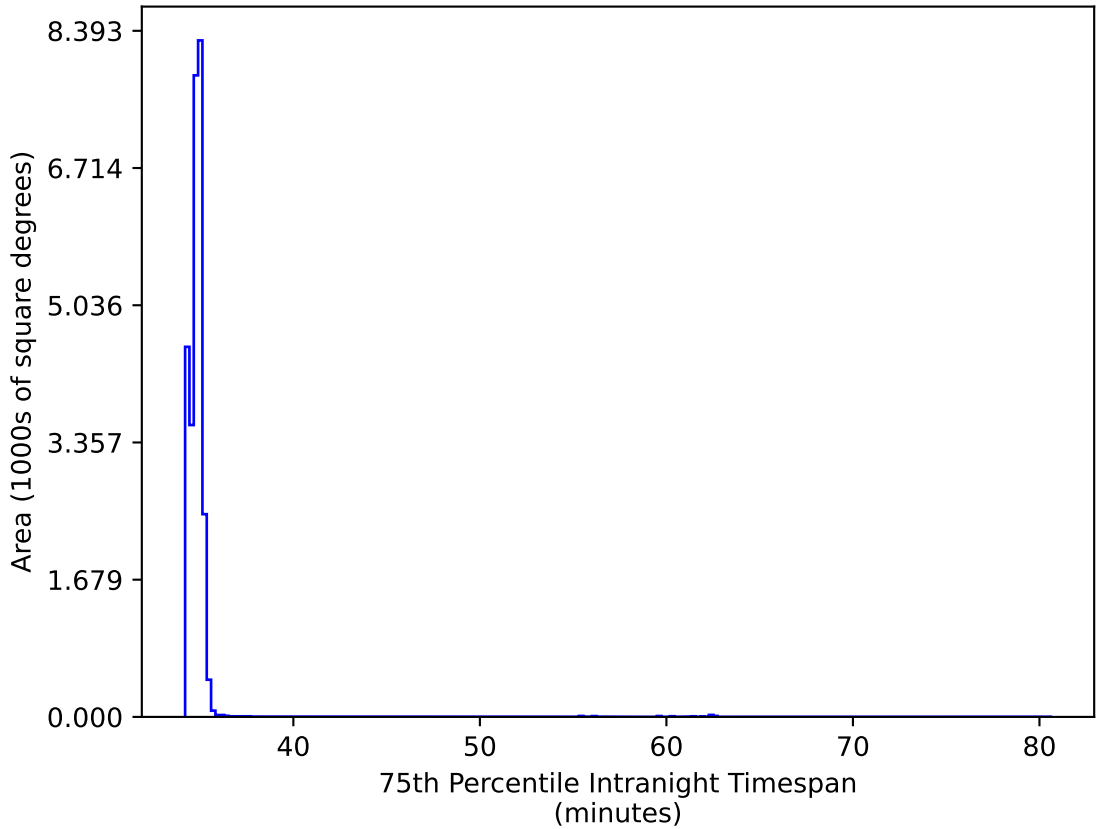
too_elab_heavy_r64_d3_griz_v3.4_10yrs All sky: 75th Percentile Intranight Timespan
