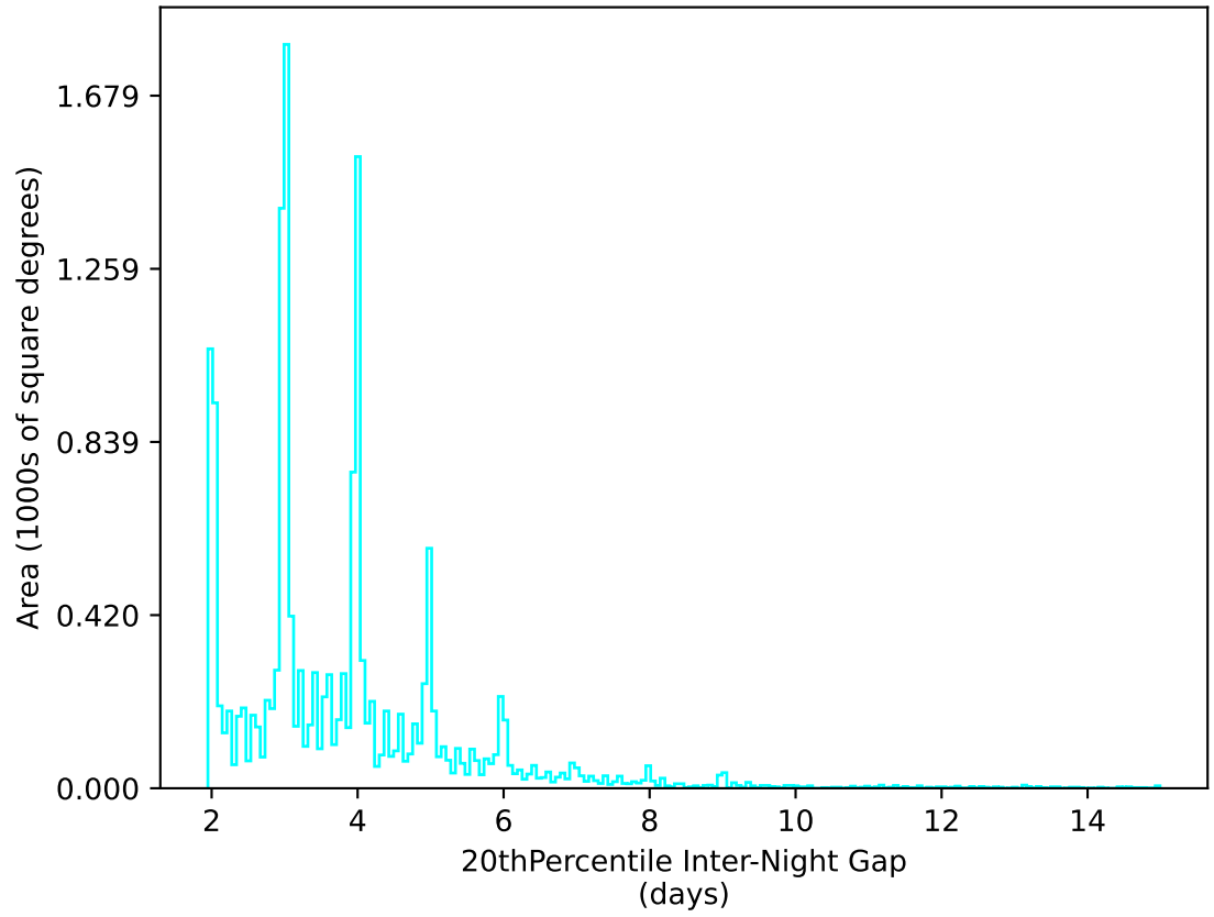
too_elab_heavy_r64_d3_griz_v3.4_10yrs WFD u band: 20thPercentile Inter-Night Gap
