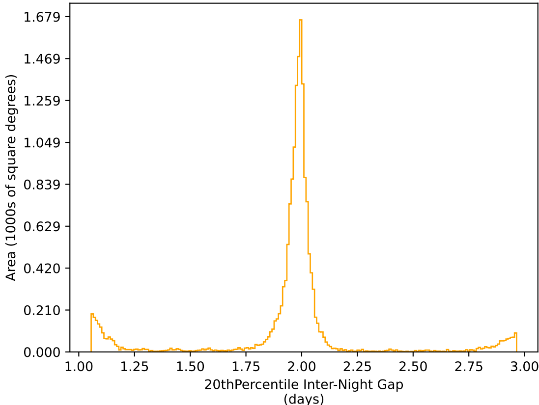
too_elab_heavy_r64_d3_griz_v3.4_10yrs WFD r band: 20thPercentile Inter-Night Gap
