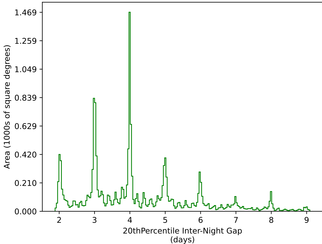
too_elab_heavy_r64_d3_griz_v3.4_10yrs WFD g band: 20thPercentile Inter-Night Gap
