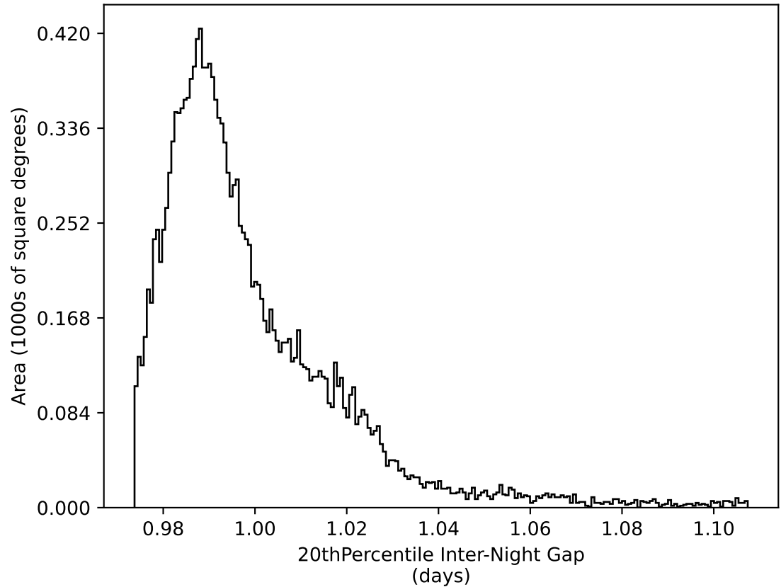
too_elab_heavy_r64_d3_griz_v3.4_10yrs WFD all bands: 20thPercentile Inter-Night Gap
