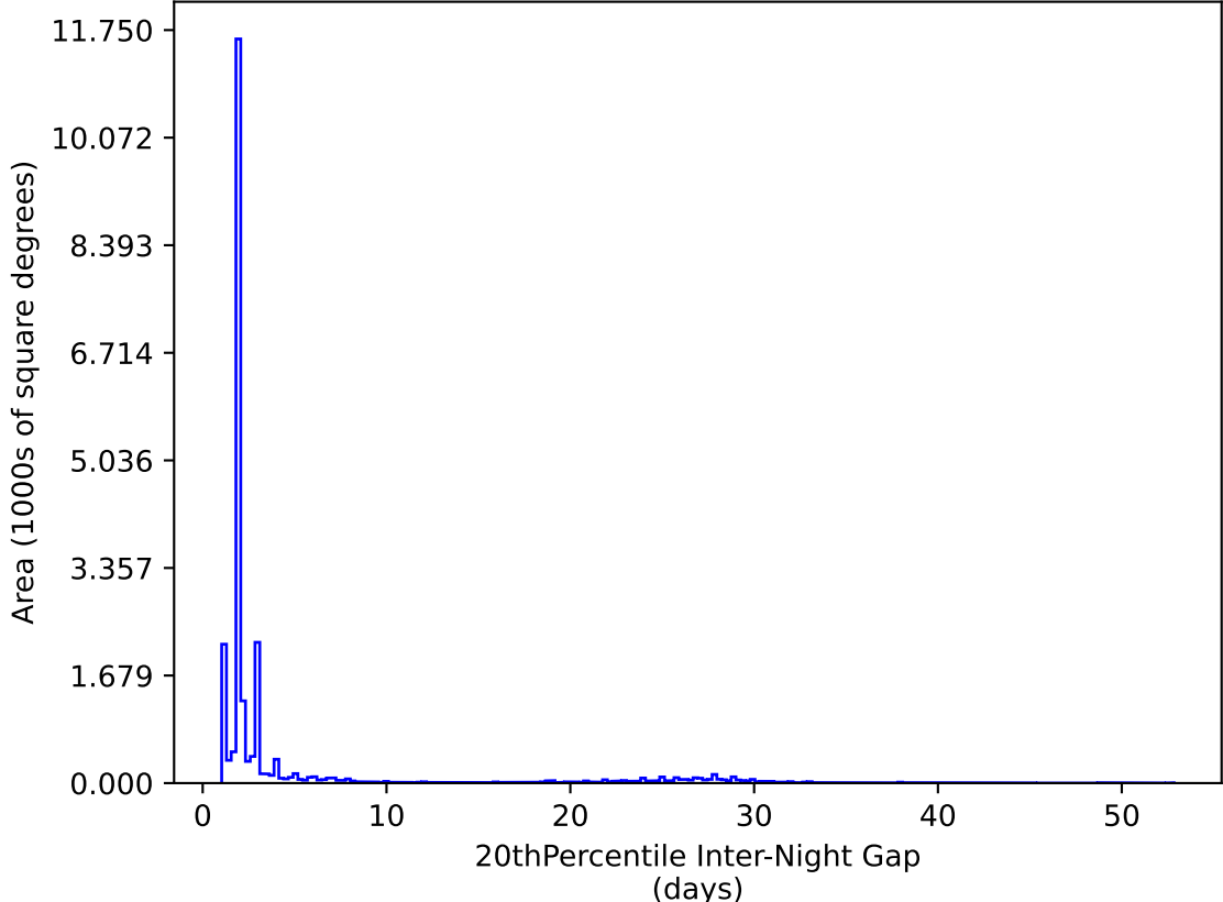
too_elab_heavy_r64_d3_griz_v3.4_10yrs All sky y band: 20thPercentile Inter-Night Gap
