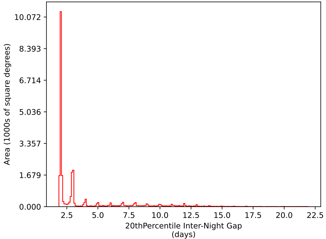
too_elab_heavy_r64_d3_griz_v3.4_10yrs All sky i band: 20thPercentile Inter-Night Gap
