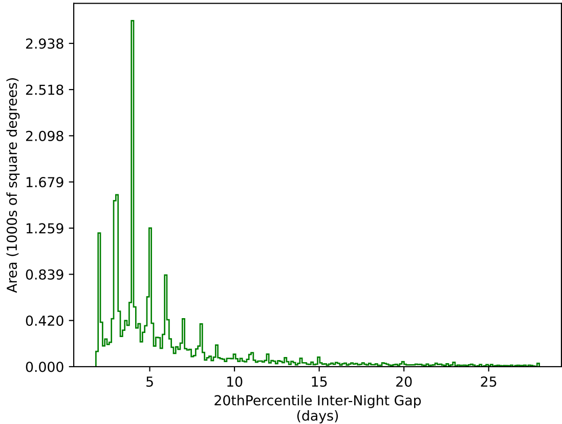
too_elab_heavy_r64_d3_griz_v3.4_10yrs All sky g band: 20thPercentile Inter-Night Gap
