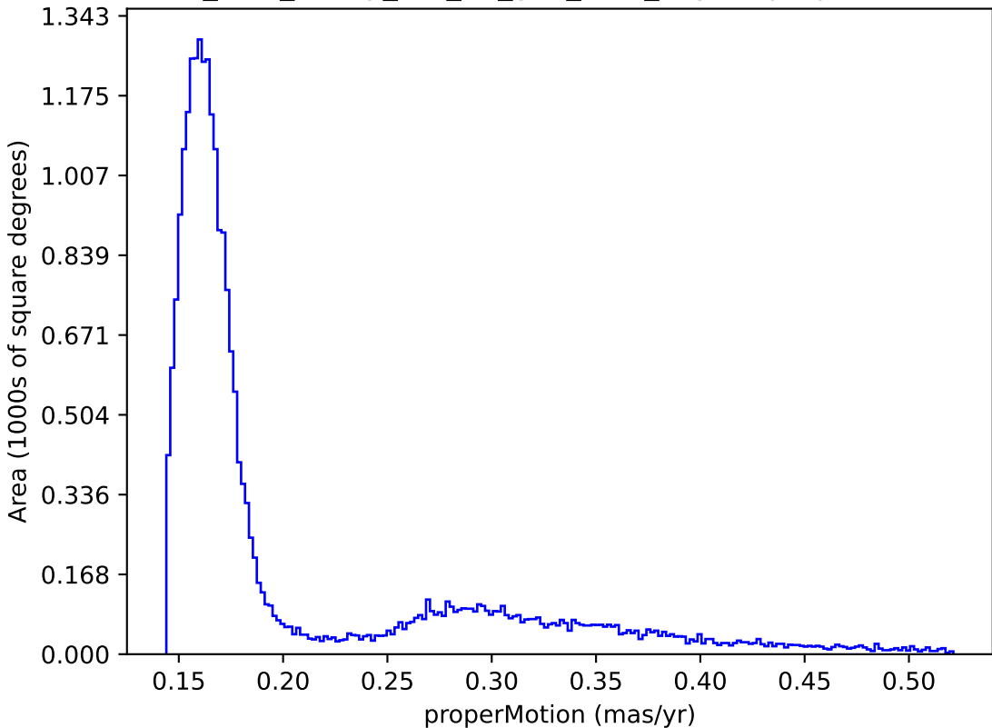
too_elab_heavy_r64_d3_griz_v3.4_10yrs : properMotion
