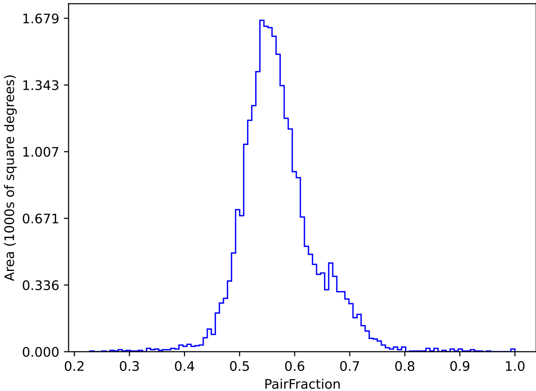
too_elab_heavy_r64_d3_griz_v3.4_10yrs (g or r or i): PairFraction
