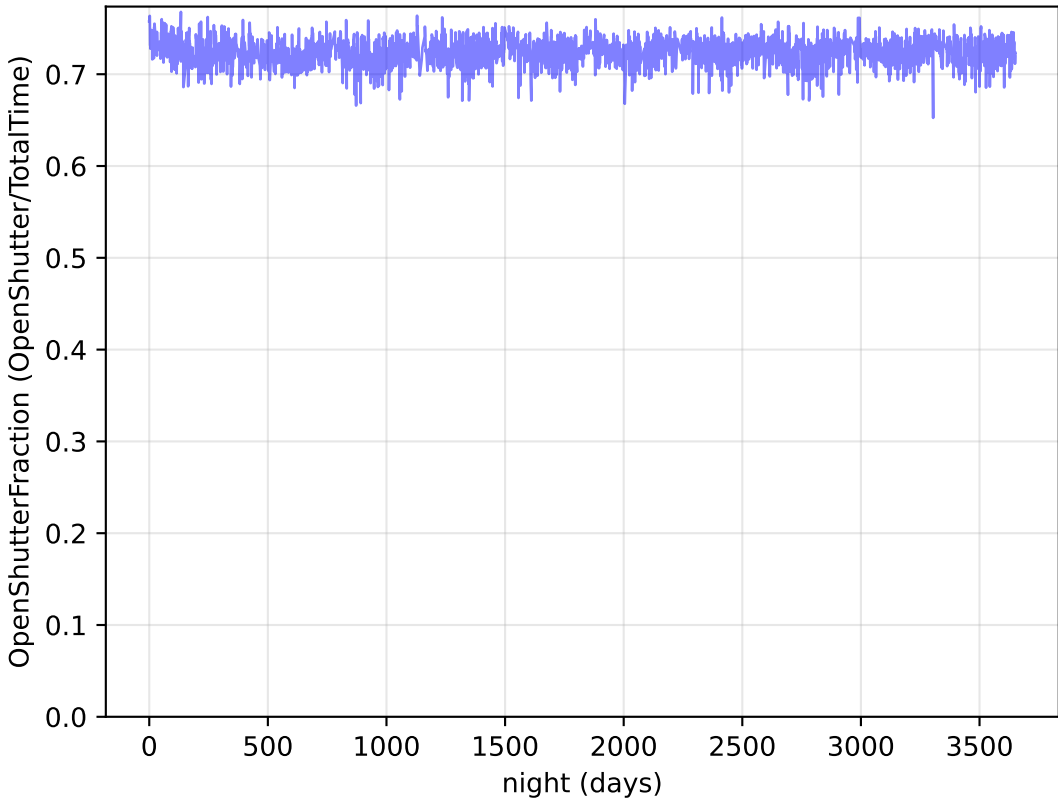
too_elab_heavy_r64_d3_griz_v3.4_10yrs : OpenShutterFraction
