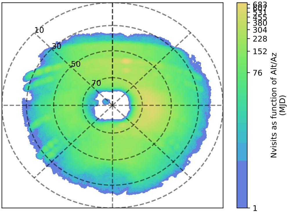
too_elab_heavy_r64_d3_griz_v3.4_10yrs u: Nvisits as function of Alt/Az
