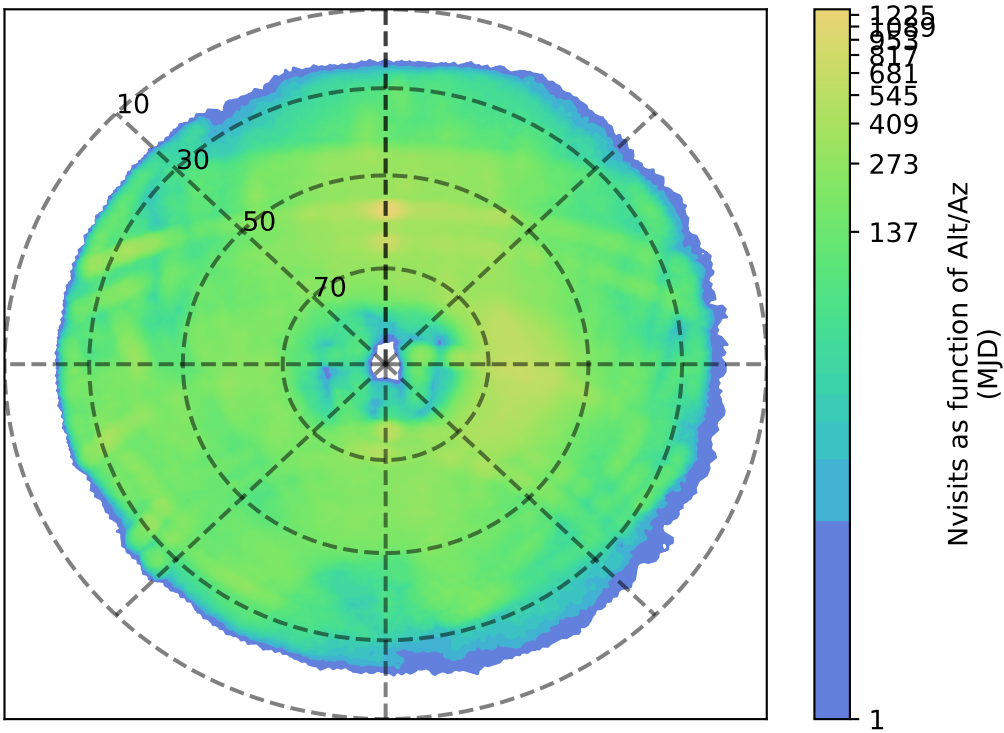
too_elab_heavy_r64_d3_griz_v3.4_10yrs g: Nvisits as function of Alt/Az
