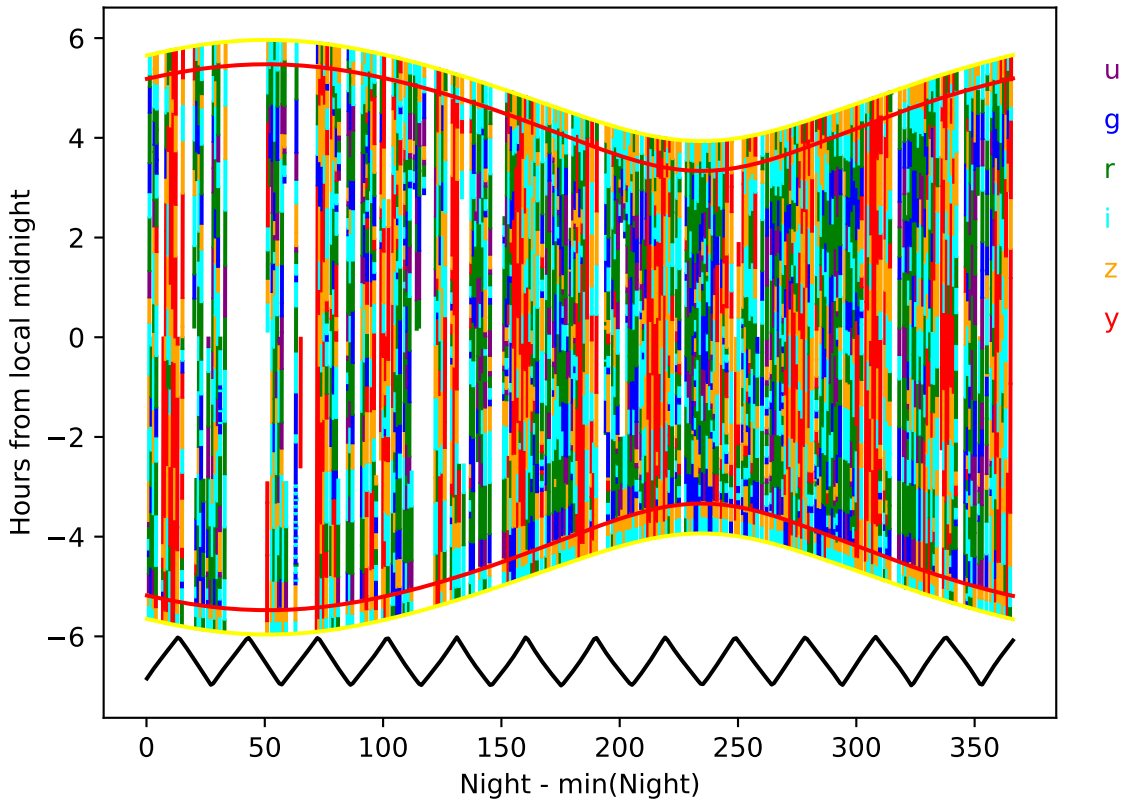
too_elab_heavy_r64_d3_griz_v3.4_10yrs year 8-9: Hourglass
