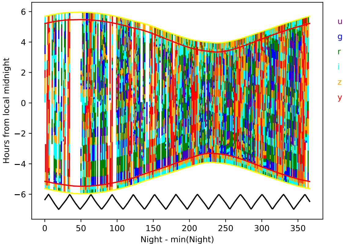
too_elab_heavy_r64_d3_griz_v3.4_10yrs year 6-7: Hourglass
