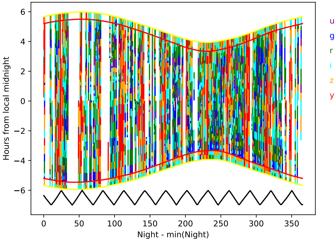
too_elab_heavy_r64_d3_griz_v3.4_10yrs year 4-5: Hourglass
