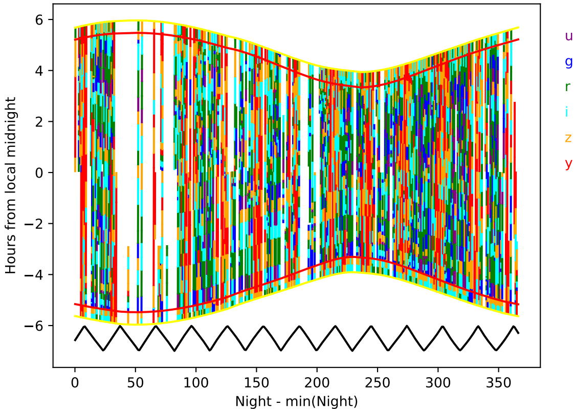
too_elab_heavy_r64_d3_griz_v3.4_10yrs year 3-4: Hourglass
