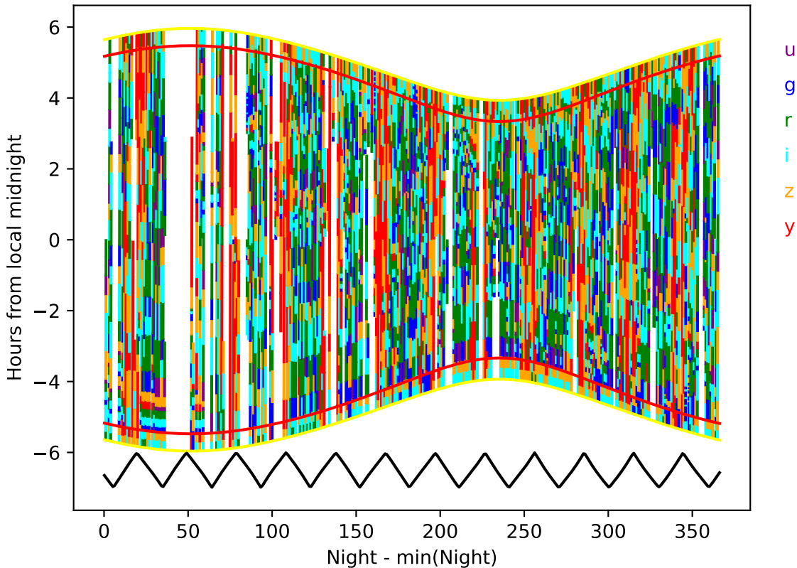
too_elab_heavy_r64_d3_griz_v3.4_10yrs year 2-3: Hourglass
