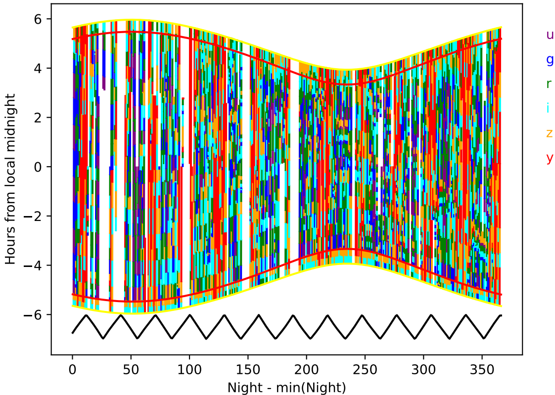
too_elab_heavy_r64_d3_griz_v3.4_10yrs year 0-1: Hourglass
