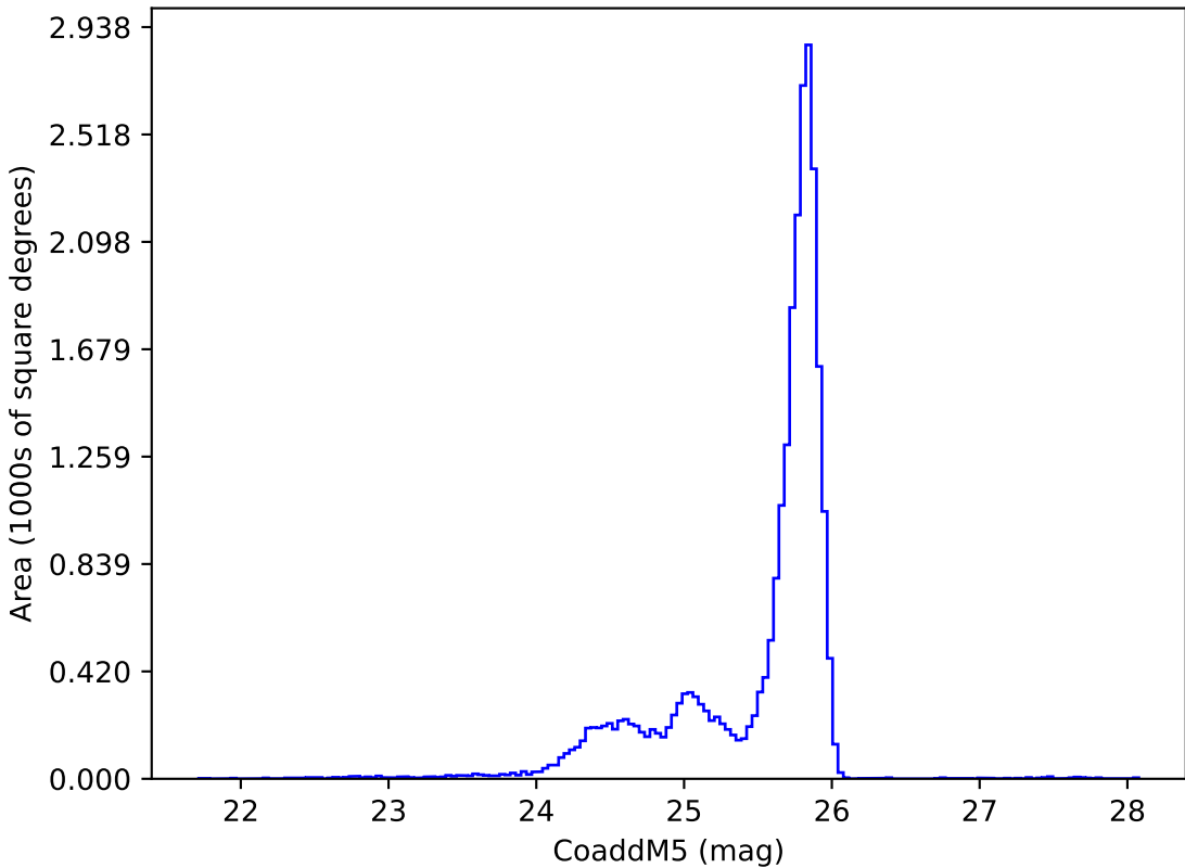
too_elab_heavy_r64_d3_griz_v3.4_10yrs z: CoaddM5
