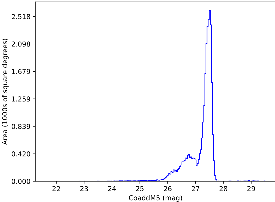
too_elab_heavy_r64_d3_griz_v3.4_10yrs : CoaddM5
