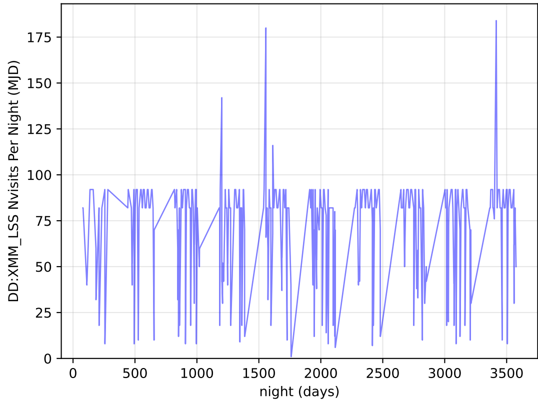
too_elab_heavy_r64_d3_griz_v3.4_10yrs all bands: DD:XMM_LSS Nvisits Per Night
