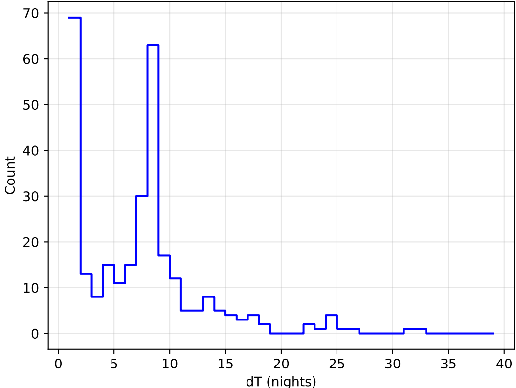
too_elab_heavy_r64_d3_griz_v3.4_10yrs all bands: DD:XMM_LSS Delta Nights Histogram
