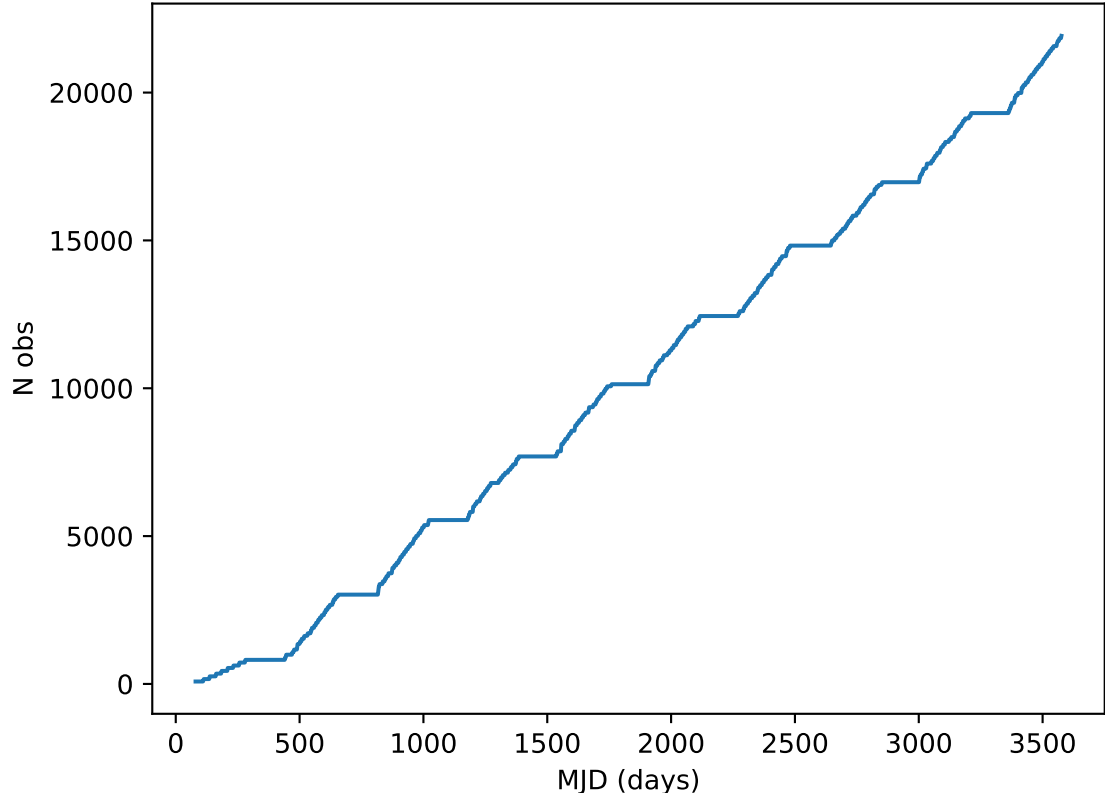
too_elab_heavy_r64_d3_griz_v3.4_10yrs all bands: DD:XMM_LSS Cumulative NVisits
