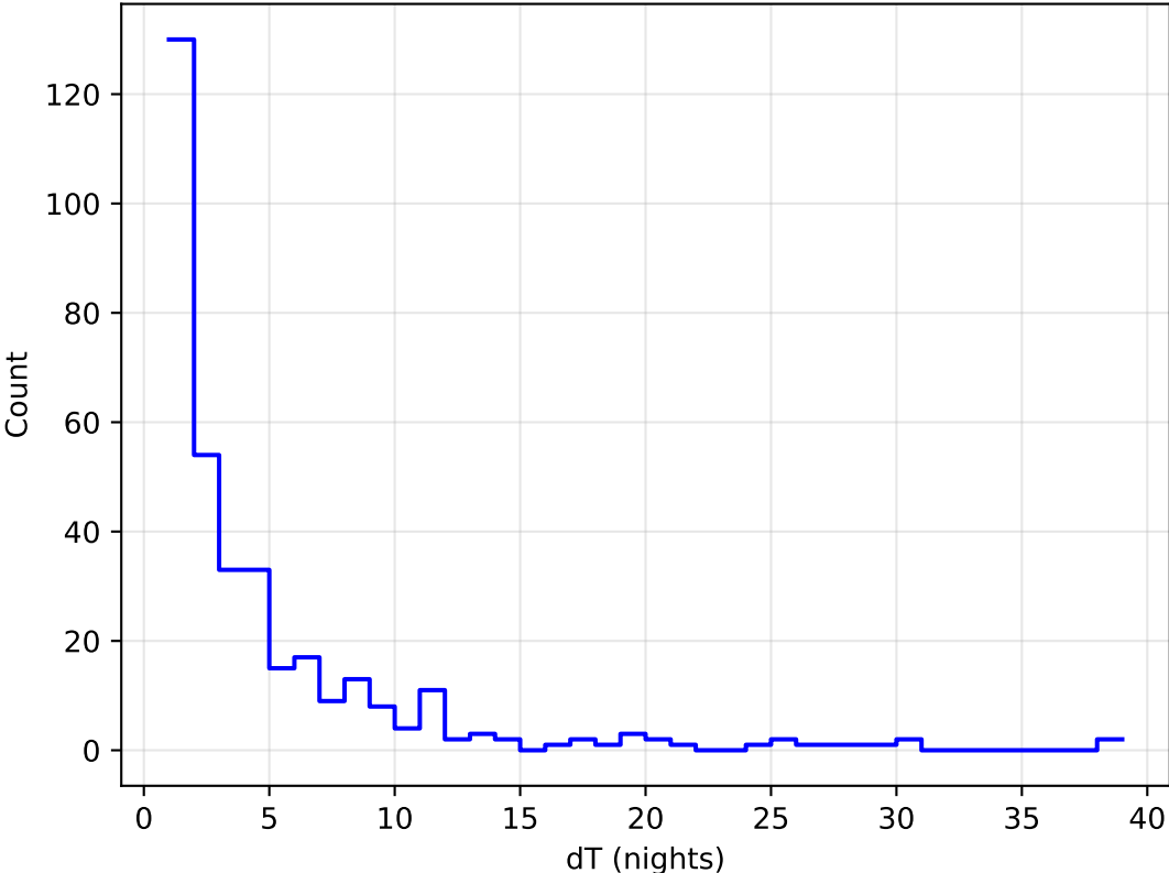
too_elab_heavy_r64_d3_griz_v3.4_10yrs all bands: DD:WFD Delta Nights Histogram
