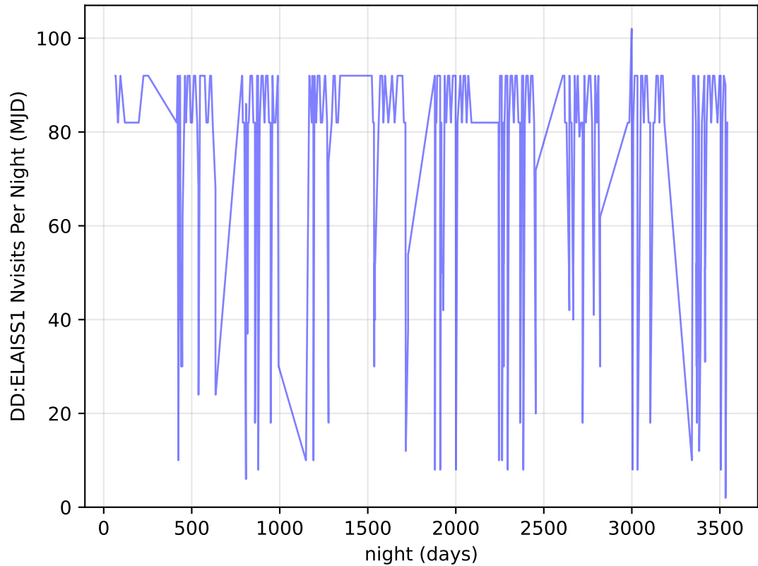
too_elab_heavy_r64_d3_griz_v3.4_10yrs all bands: DD:ELAISS1 Nvisits Per Night
