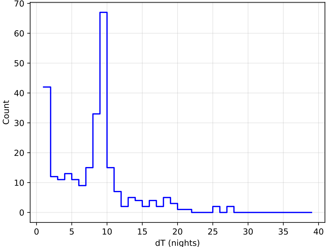
too_elab_heavy_r64_d3_griz_v3.4_10yrs all bands: DD:ELAISS1 Delta Nights Histogram
