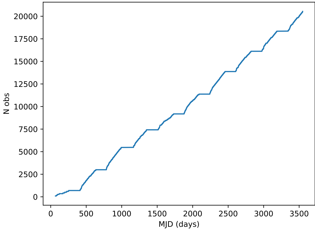
too_elab_heavy_r64_d3_griz_v3.4_10yrs all bands: DD:ELAISS1 Cumulative NVisits
