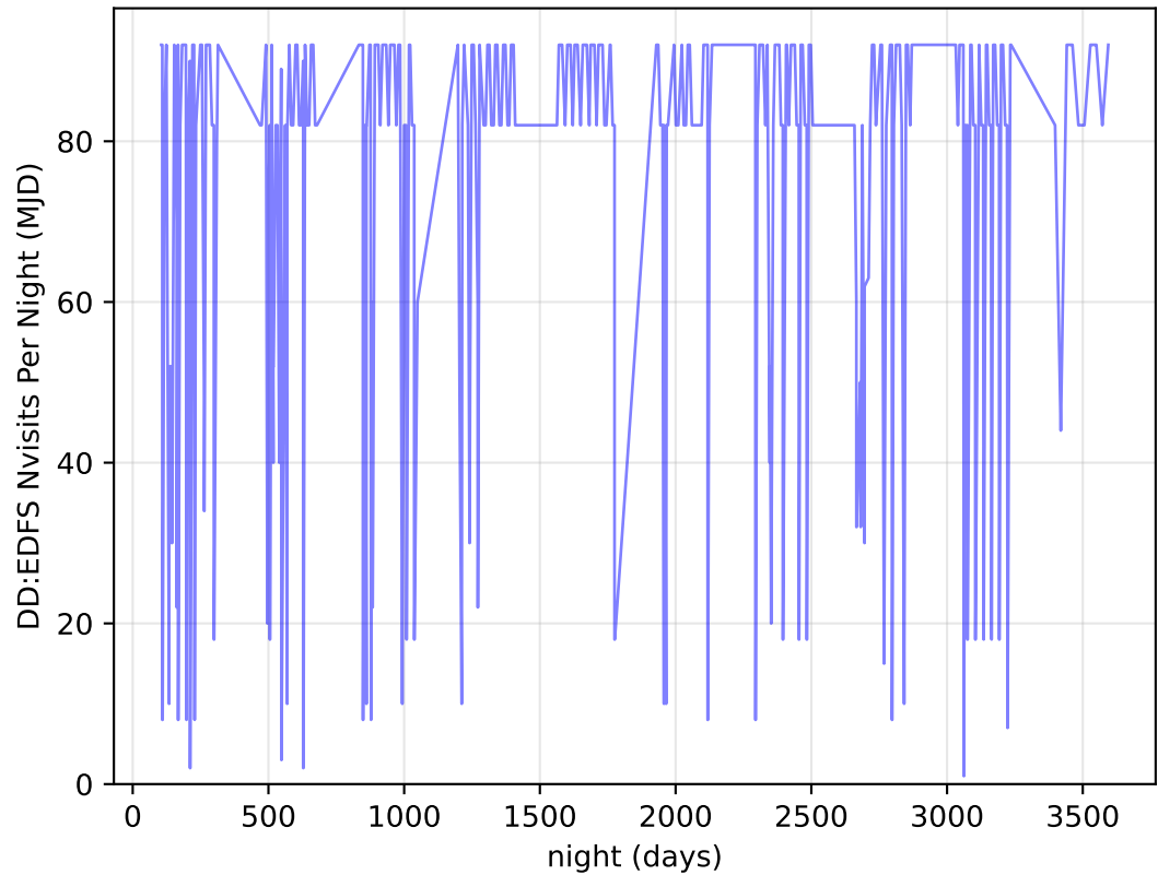
too_elab_heavy_r64_d3_griz_v3.4_10yrs all bands: DD:EDFS Nvisits Per Night
