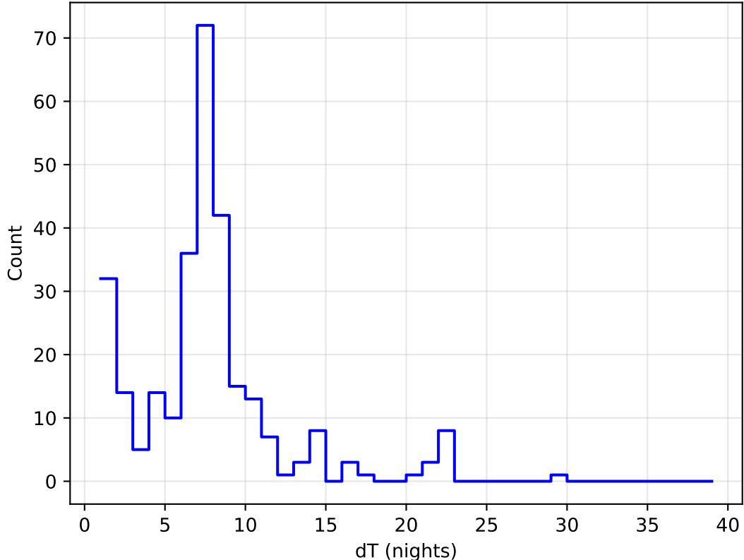
too_elab_heavy_r64_d3_griz_v3.4_10yrs all bands: DD:EDFS Delta Nights Histogram
