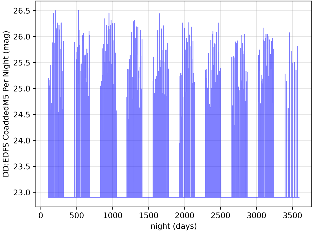
too_elab_heavy_r64_d3_griz_v3.4_10yrs r band: DD:EDFS CoaddedM5 Per Night
