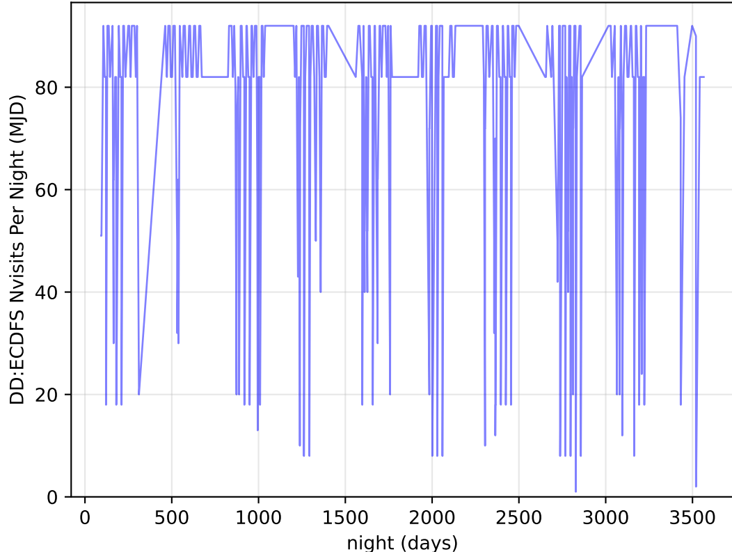
too_elab_heavy_r64_d3_griz_v3.4_10yrs all bands: DD:ECDFS Nvisits Per Night
