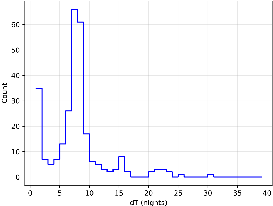
too_elab_heavy_r64_d3_griz_v3.4_10yrs all bands: DD:ECDFS Delta Nights Histogram
