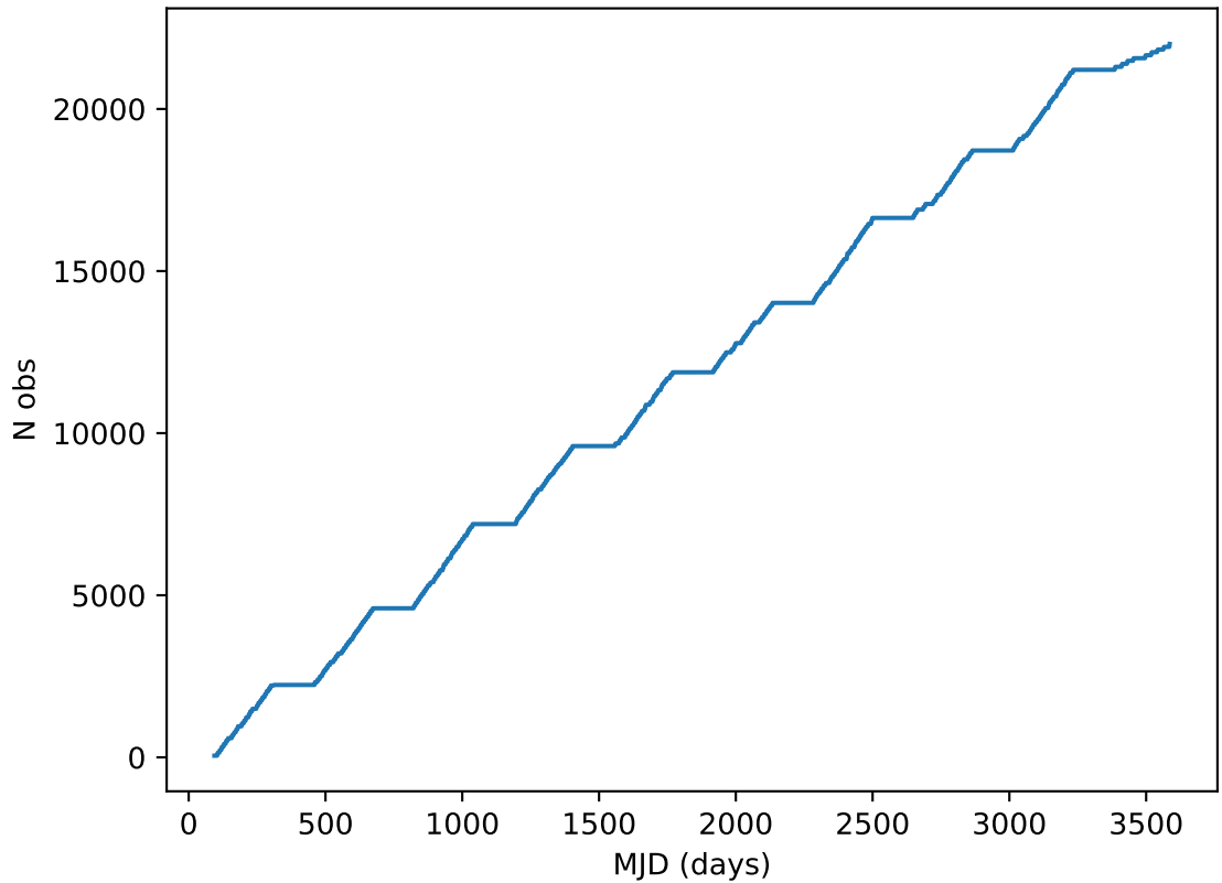
too_elab_heavy_r64_d3_griz_v3.4_10yrs all bands: DD:ECDFS Cumulative NVisits
