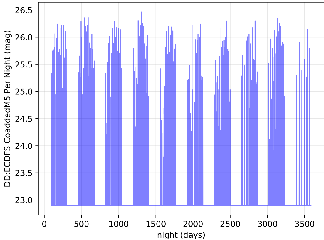
too_elab_heavy_r64_d3_griz_v3.4_10yrs r band: DD:ECDFS CoaddedM5 Per Night
