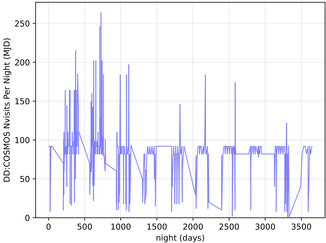
too_elab_heavy_r64_d3_griz_v3.4_10yrs all bands: DD: COSMOS Nvisits Per Night
