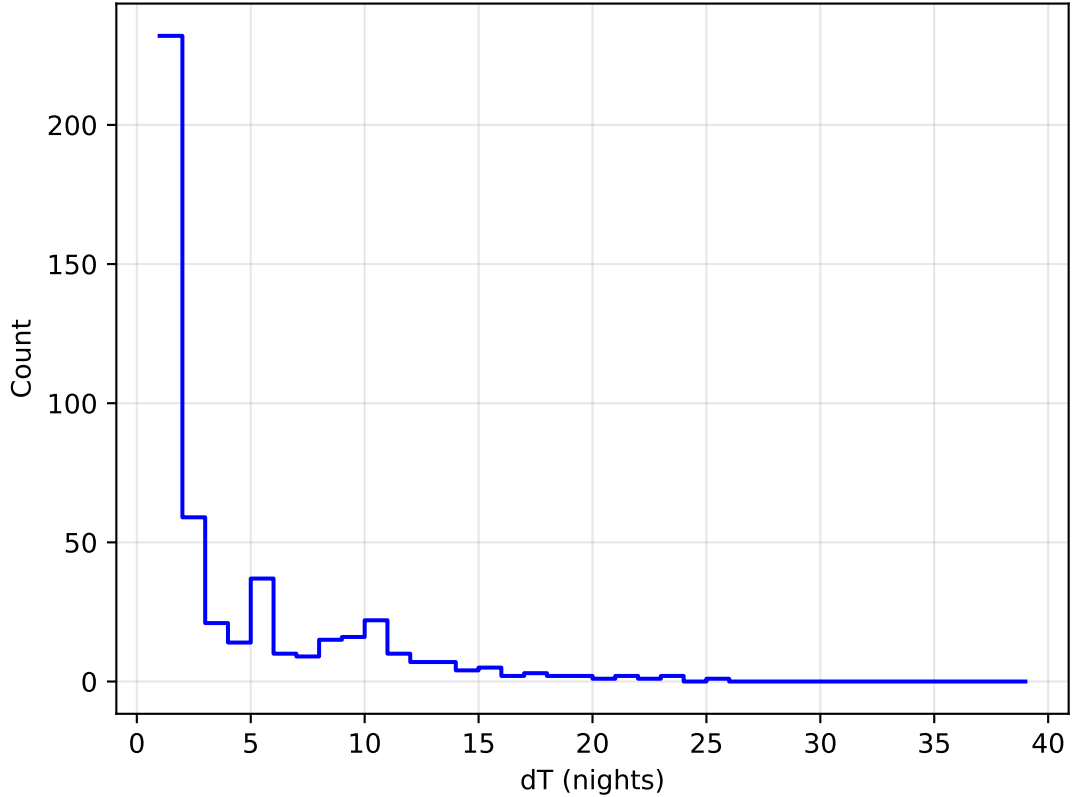
too_elab_heavy_r64_d3_griz_v3.4_10yrs all bands: DD: COSMOS Delta Nights Histogram
