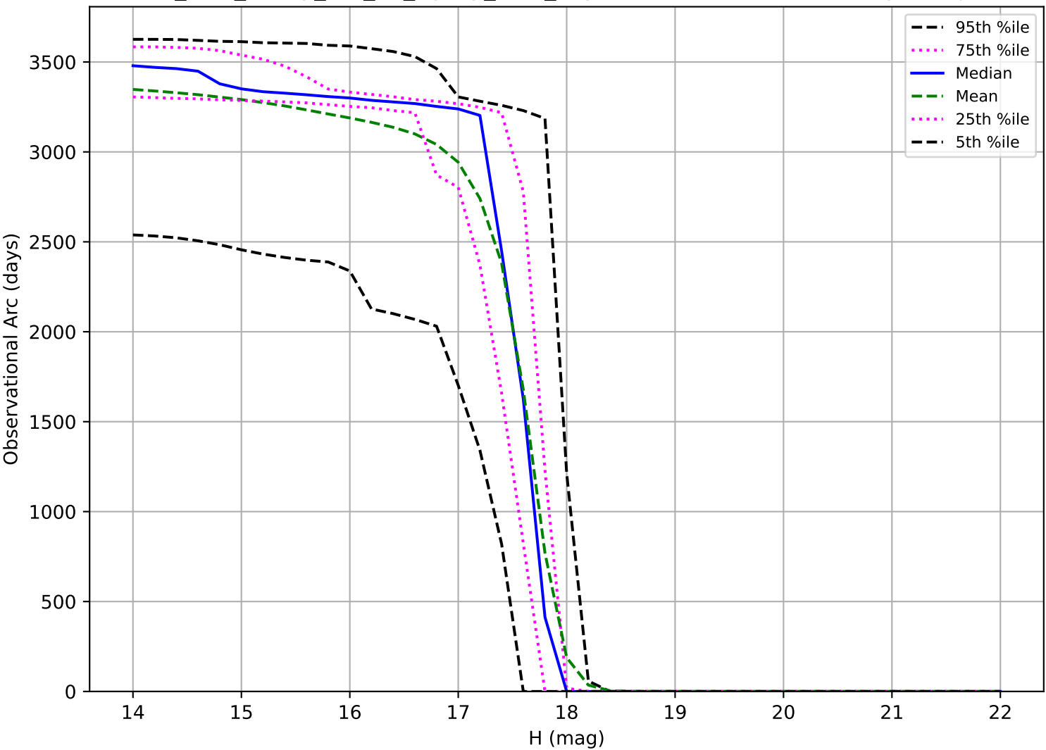
too_elab_heavy_r64_d2_ugrizy_v3.4_10yrs: Observational Arc Length Trojan
