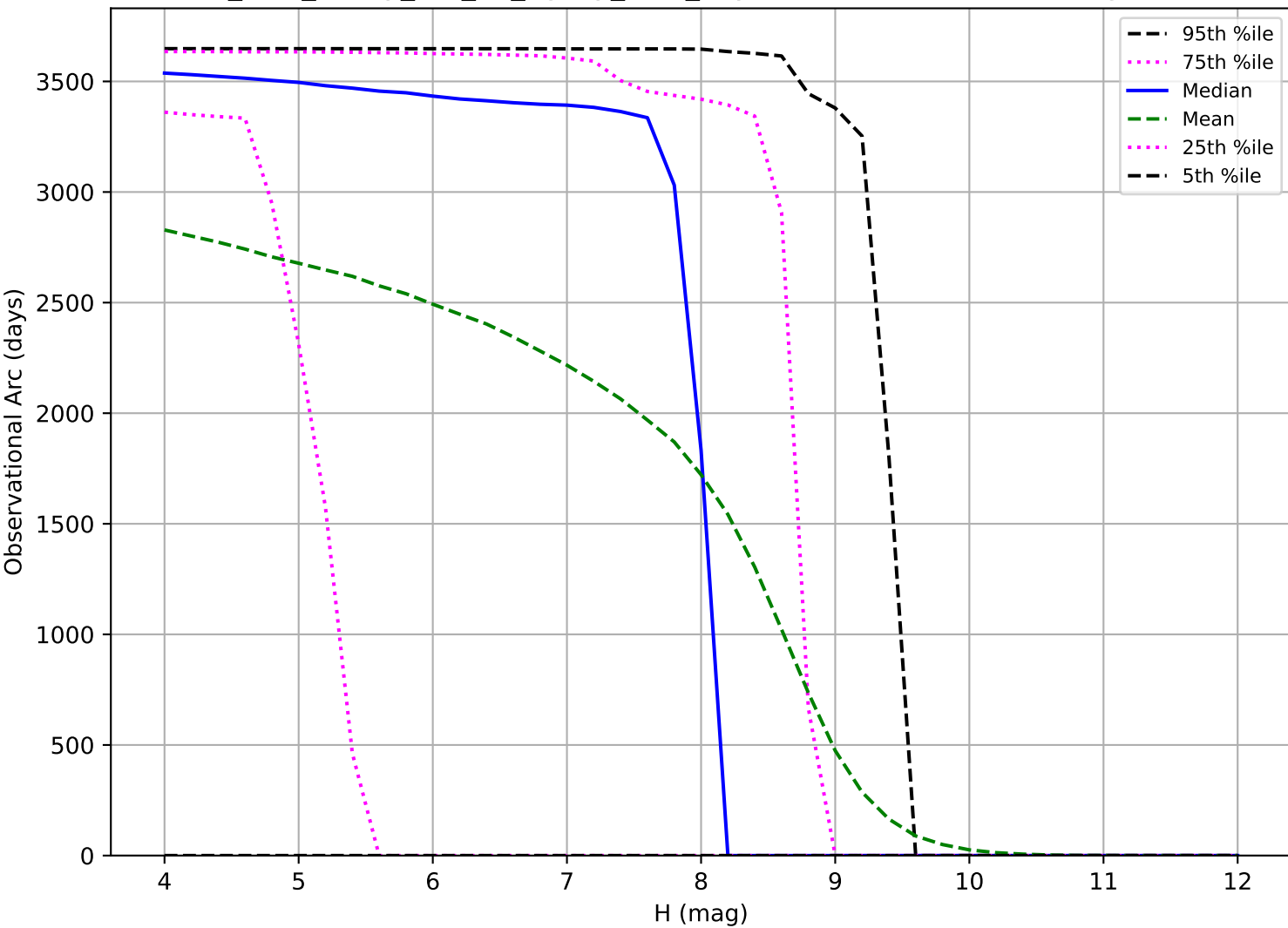
too_elab_heavy_r64_d2_ugrizy_v3.4_10yrs: Observational Arc Length TNO
