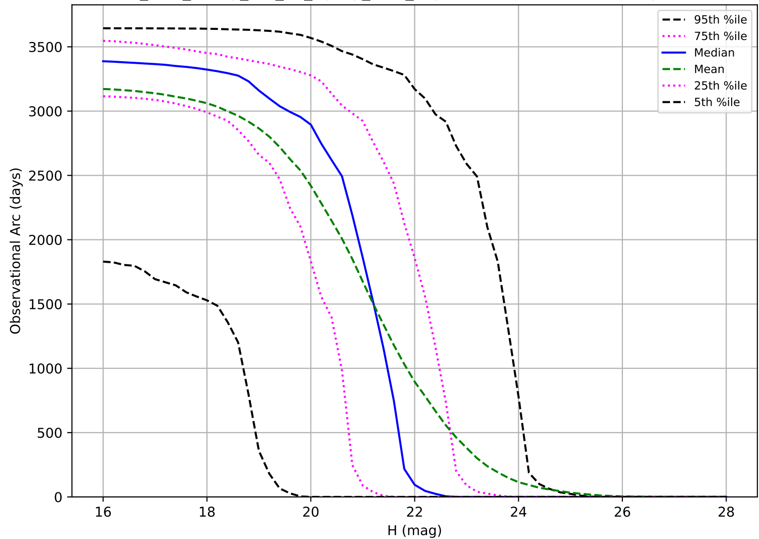
too_elab_heavy_r64_d2_ugrizy_v3.4_10yrs: Observational Arc Length NEO
