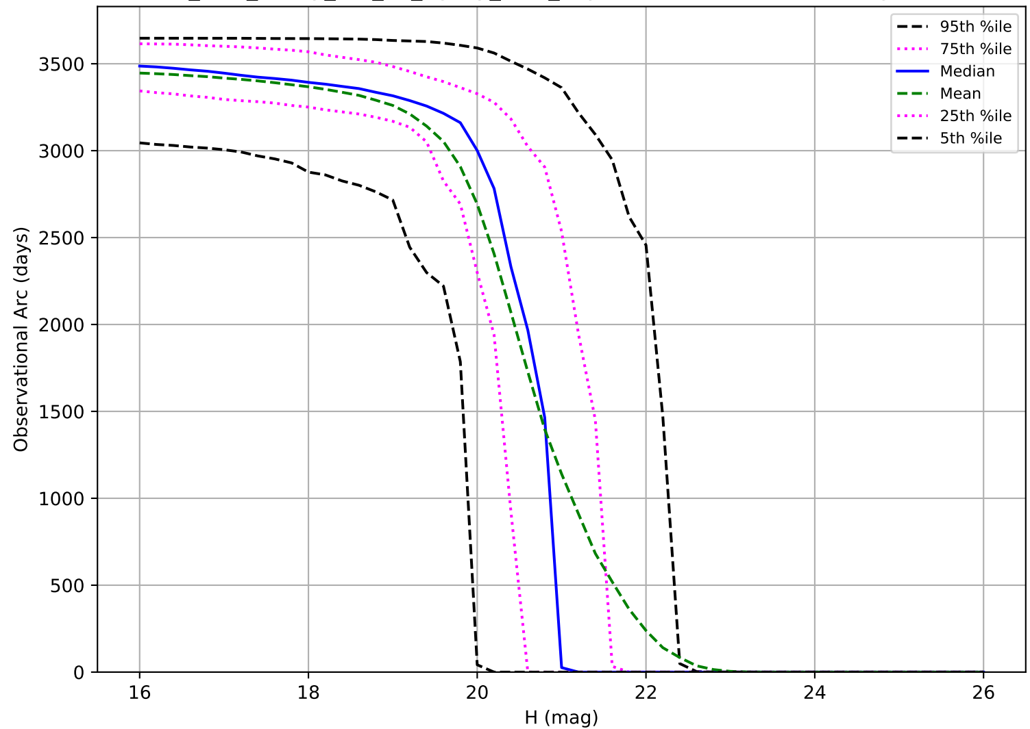
too_elab_heavy_r64_d2_ugrizy_v3.4_10yrs: Observational Arc Length MBA
