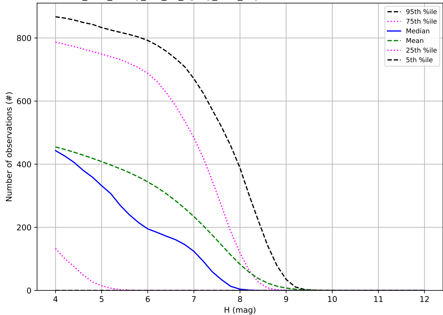
too_elab_heavy_r64_d2_ugrizy_v3.4_10yrs: Number of observations TNO
