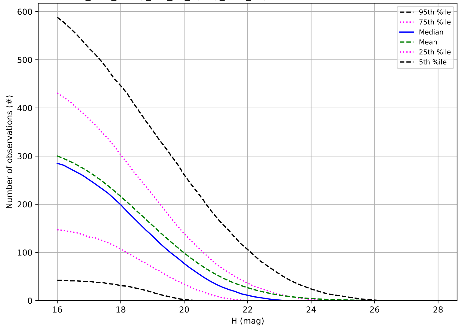
too_elab_heavy_r64_d2_ugrizy_v3.4_10yrs: Number of observations PHA
