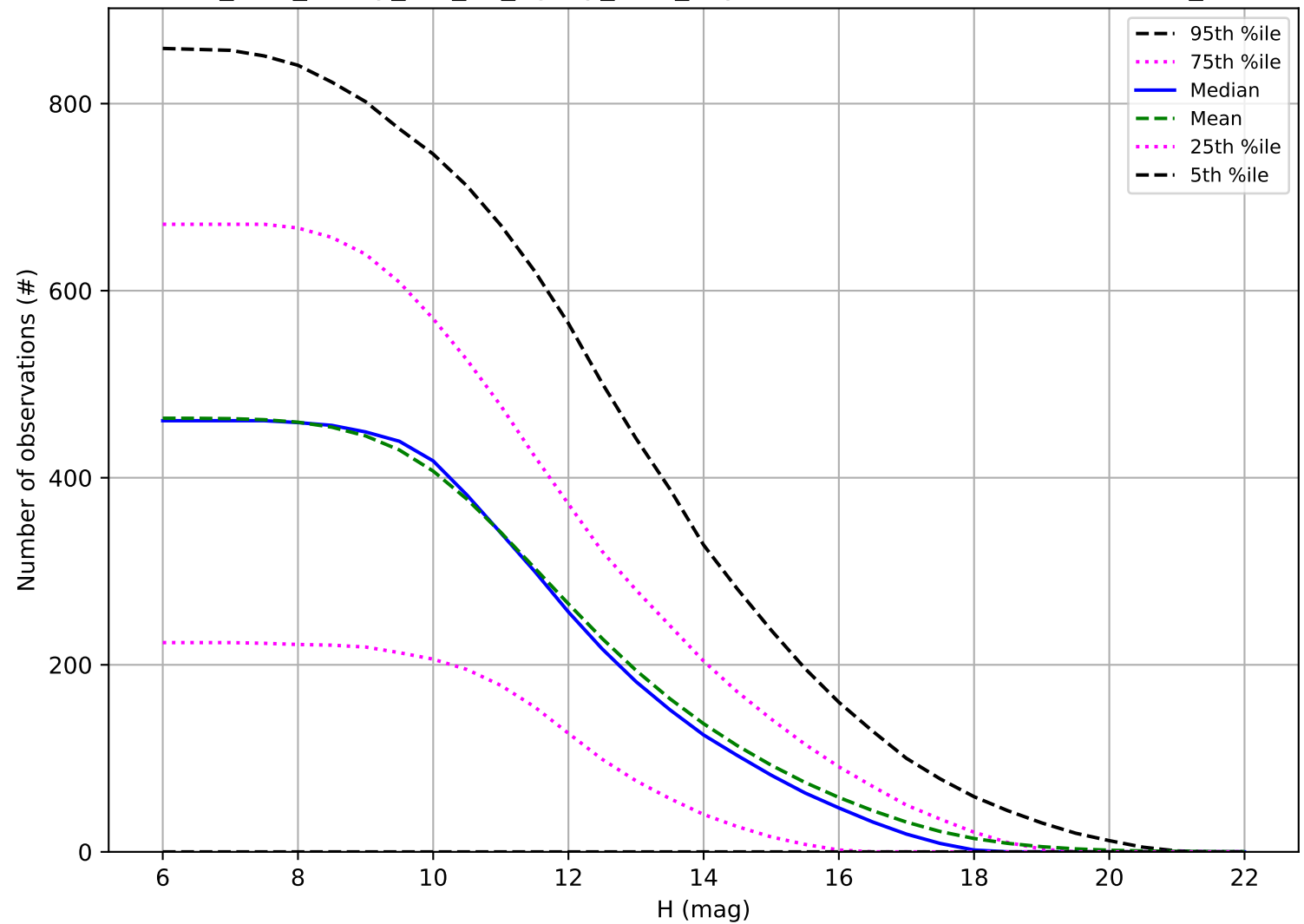
too_elab_heavy_r64_d2_ugrizy_v3.4_10yrs: Number of observations OCC_r5
