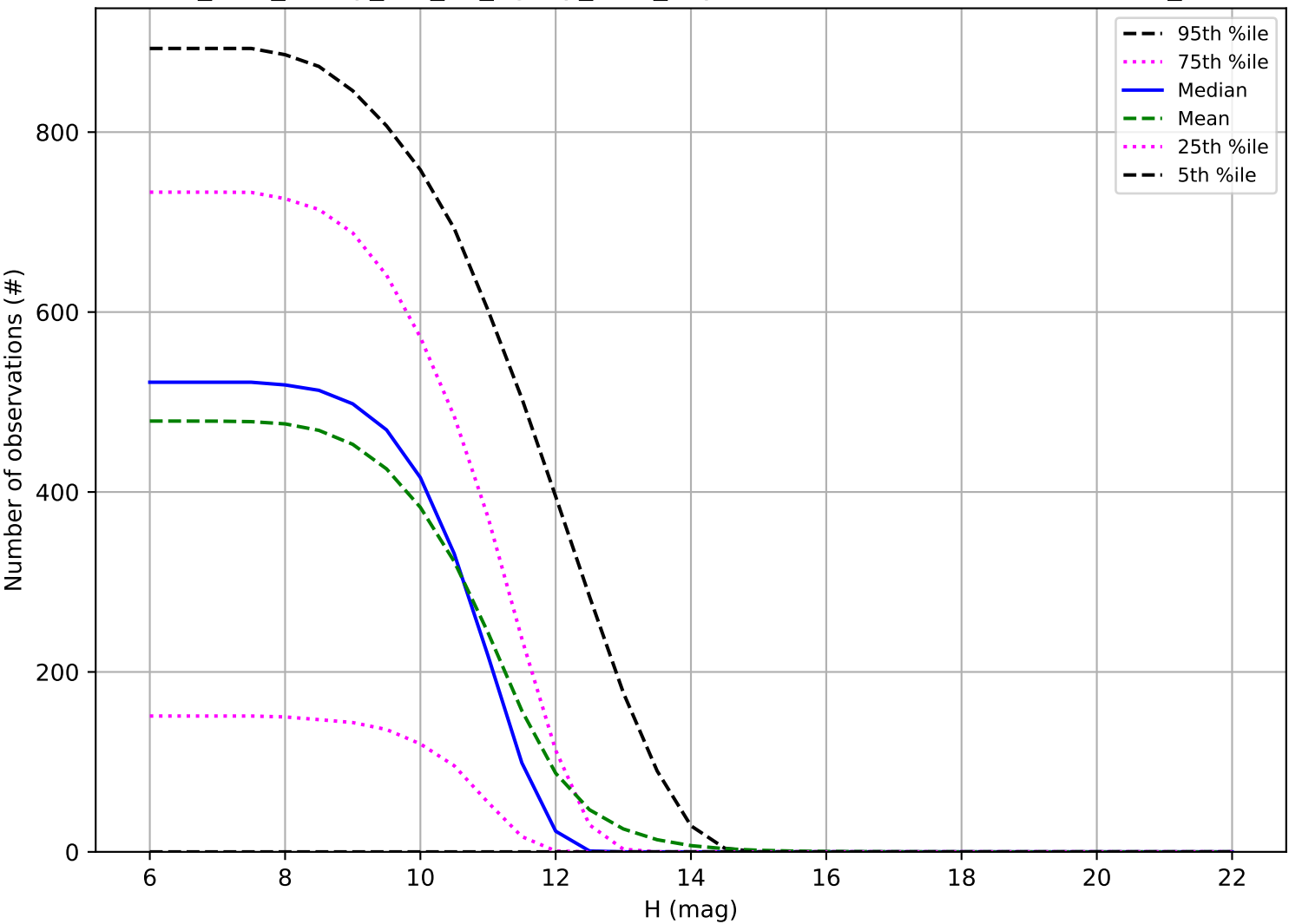
too_elab_heavy_r64_d2_ugrizy_v3.4_10yrs: Number of observations OCC_r20
